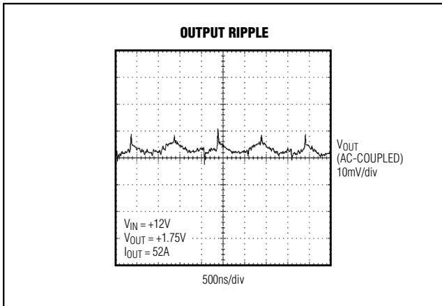
Figure 7. Output Ripple
