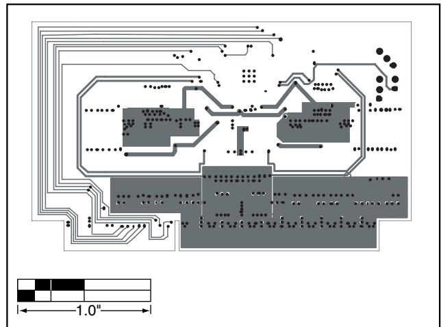
Figure 22. MAX5037 EV Kit PC Board Layout—Inner Layer 3
