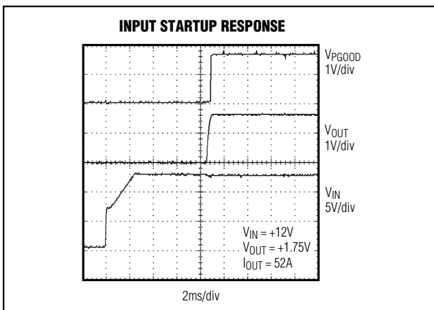
Figure 13. Input Startup Response
