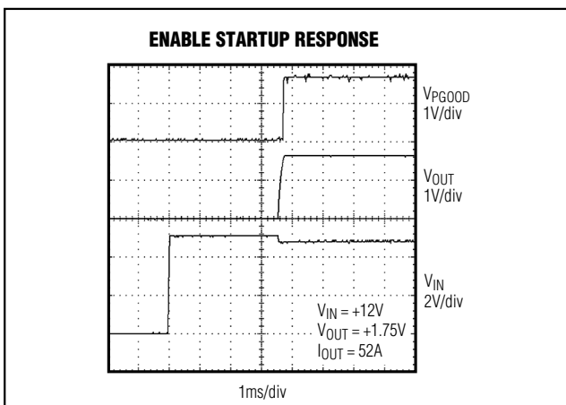
Figure 14. Enable Startup Response
