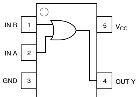
Figure 1. Pinout
