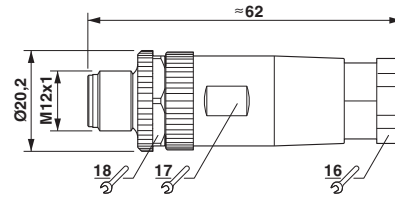
M12 x 1 plug, straight
