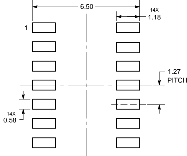
DIMENSIONS: MILLIMETERS
