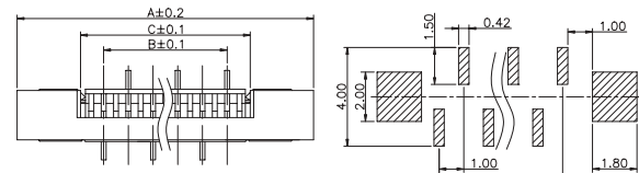
PCB LAYOUT - COMPONENT VIEW
