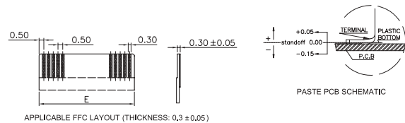
APPLICABLE FFC LAYOUT (THICKNESS: 0,3 ±0,05)
