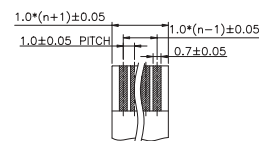
APPLICABLE FFC LAYOUT (THICKNESS: 0.3 ± 0.05)
