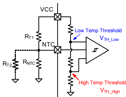
Figure 9—NTC Function Block
