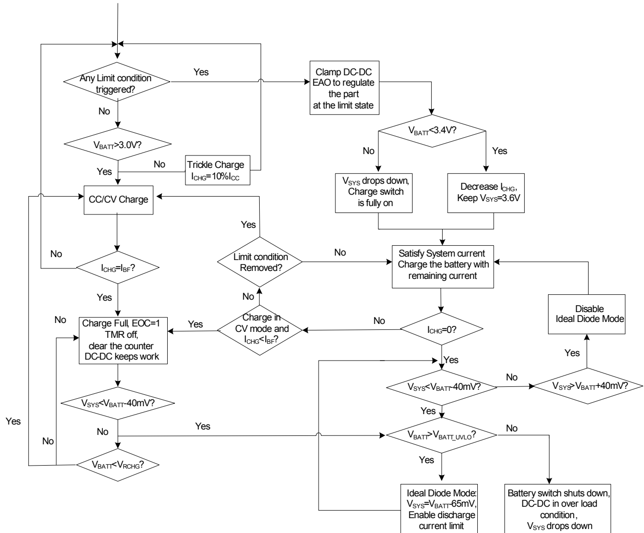
Figure 6— MP2617B Operation Flow Chart under No Fault Condition
