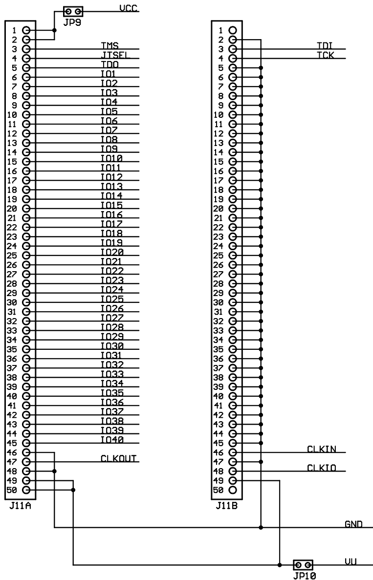
FX2 Connector
