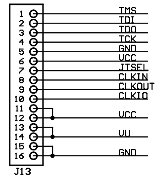
FX2 Connector JTAG and Clock Signals
