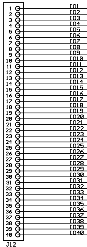
FX2 Connector I/O Signals
