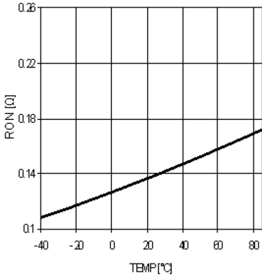
Fig.8 Hi,Low-Side On-resistance
