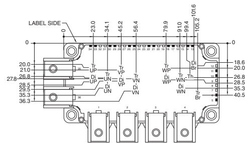
Each mark points to the center position of each chip. T^*P / T^*N / T^*Br (* = U/V/W): IGBT D^*P / D^*N (* = U/V/W): FWDi DiBr: Clamp Th: NTC Thermistor
